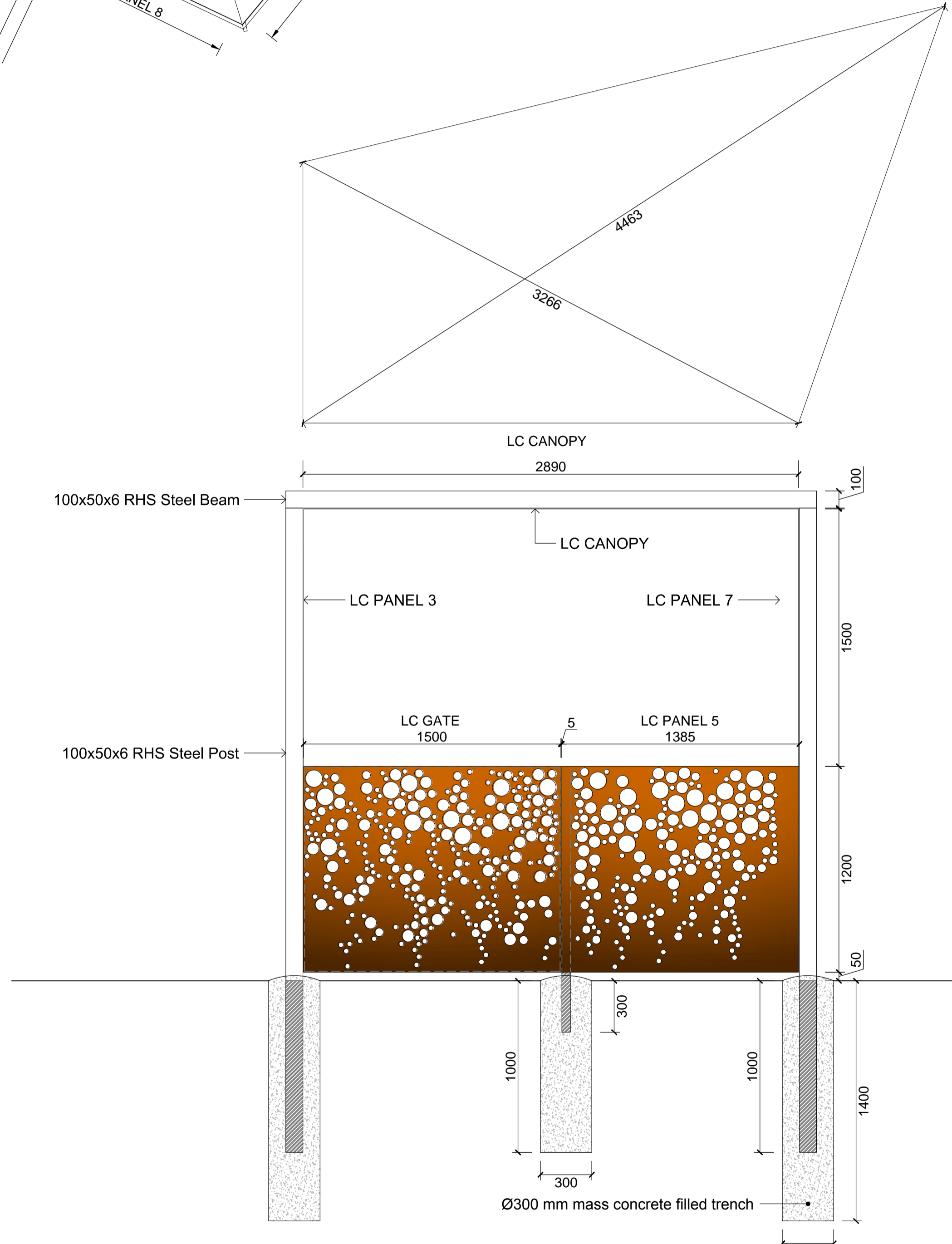
56 LASER CUT METAL FENCE, SCREEN & CANOPY L-015 Detailed Elevation 2 Scale 1:20
