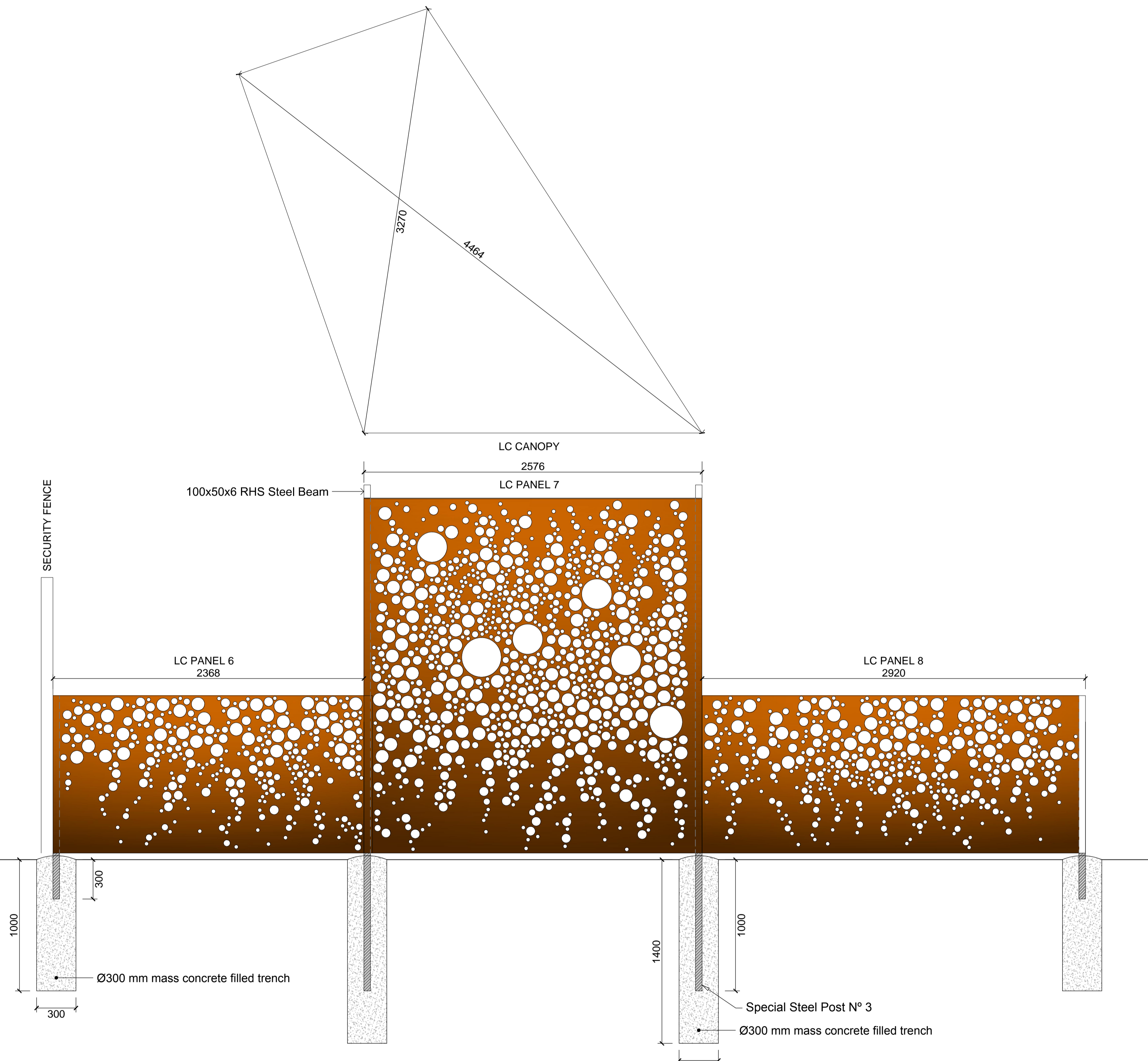
57 LASER CUT METAL FENCE, SCREEN & CANOPY L-015 Detailed Elevation 3 Scale 1:20
